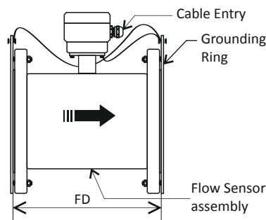
Fig. 5 Front View
