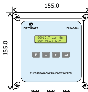
Fig. 3 Front View
