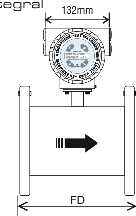
Fig. 1 Front View
