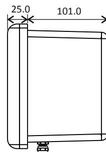
Fig. 4 Side View
