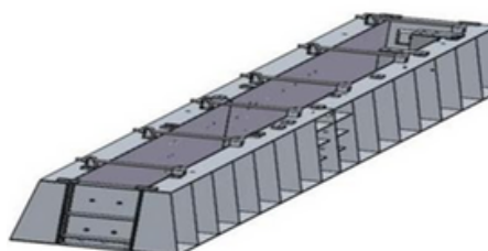
I-Girder Mould
